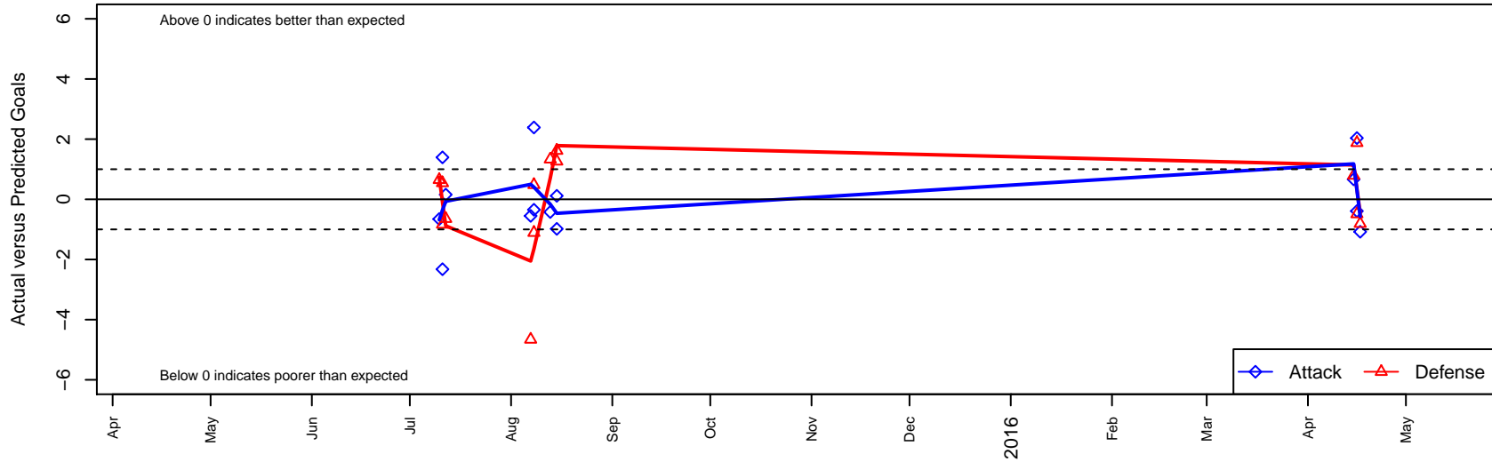
Kent United Green G97 Dots are actual minus expected GF (blue circles) and GA (red triangles). Blue line is smoothed change in attack strength. Red is smoothed change in defense strength.
